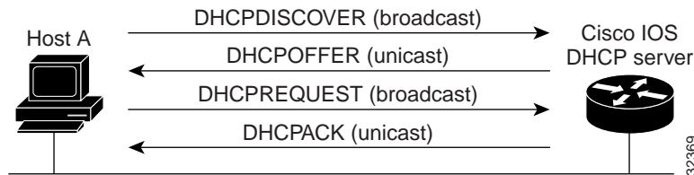
Figure 15 DHCP Request for an IP Address from a DHCP Server
